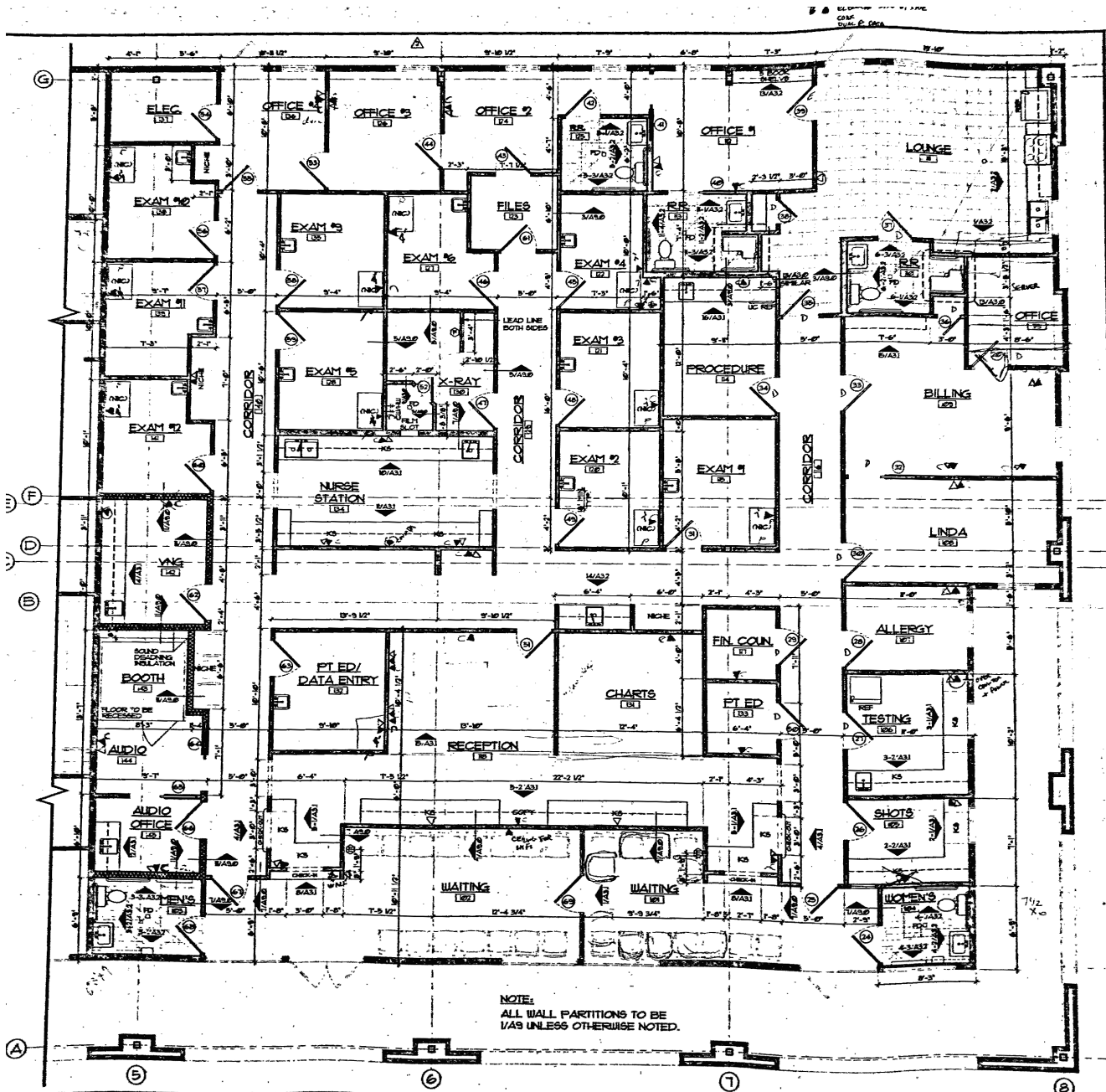
Space 1 Floor Plan 5,821 SF (Possible to combine with Space 2)
